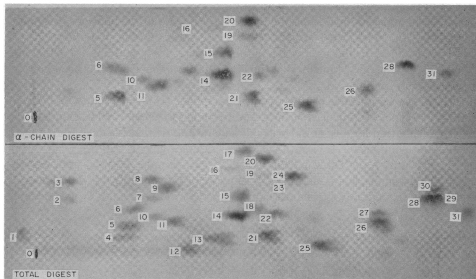
FIG. 3.—Peptide maps of tryptic digest of total rabbit globin (bottom) and column separated \alpha -chain (top). The point of application of digest to the paper is marked by O. The positive electrode is to the left.
