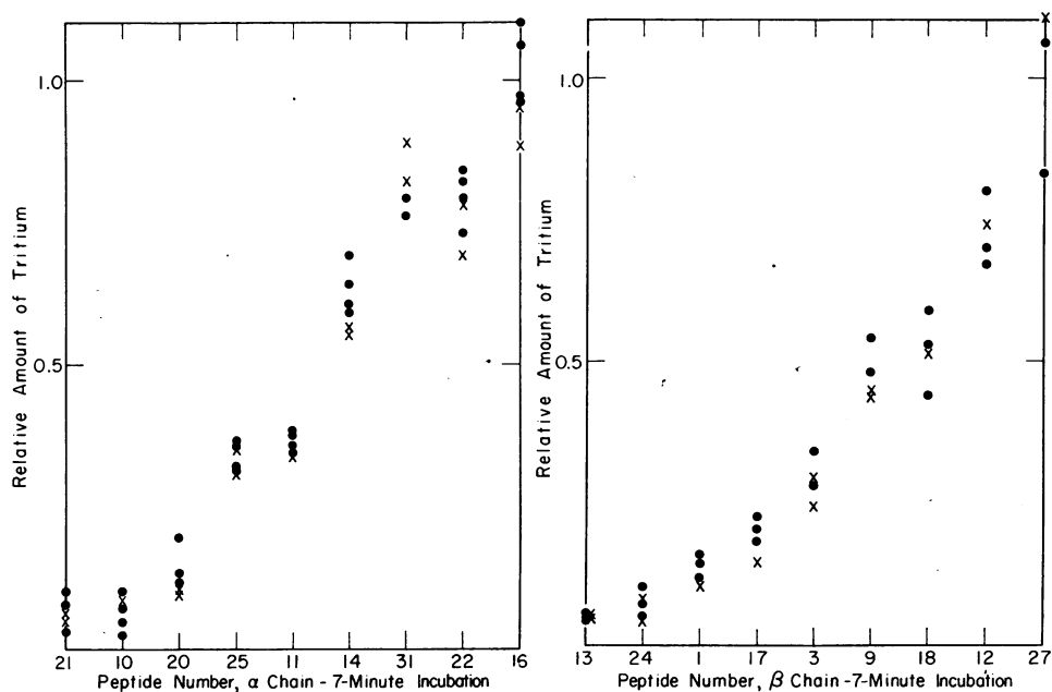
FIG. 4.—Distribution of H^3 -leucine among tryptic peptides of soluble rabbit hemoglobin. Peptides produced by tryptic digestion in an autotitrator are indicated by ●. Peptides produced from a separate incubation by tryptic digestion in buffer are indicated by X.
