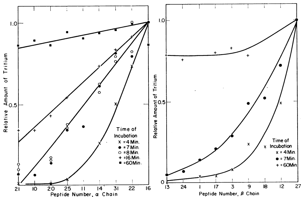
FIG. 5.—Distribution of H^3 -leucine among tryptic peptides of soluble rabbit hemoglobin after various times of incubation at 15^\circ\text{C} . The points indicated for 7 minutes (●) are the result of averaging all points shown in Figure 4.
