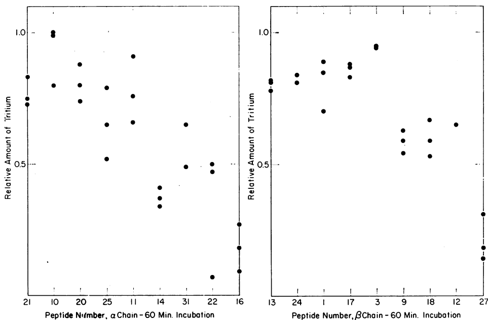
FIG. 7.—Distribution of H^3 -leucine among tryptic peptides of ribosomes after long incubations.
