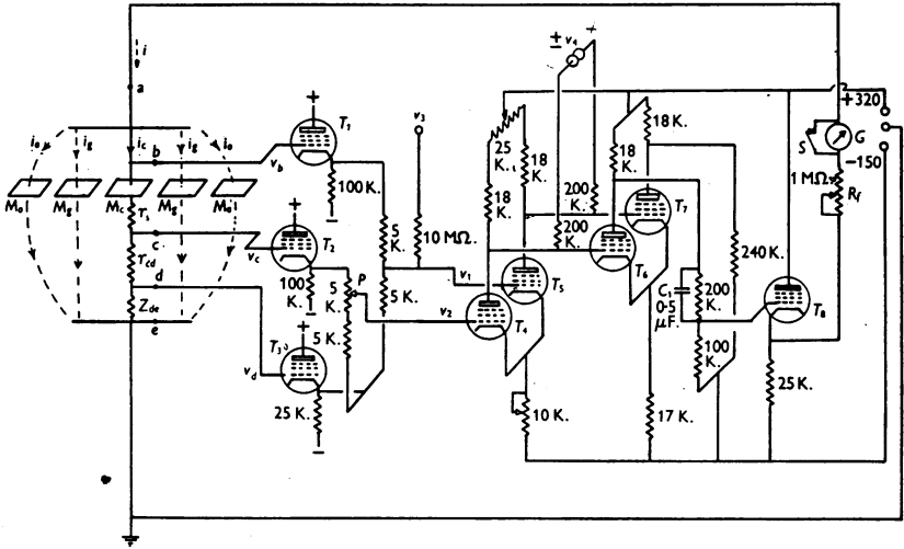
Fig. 6. Schematic diagram of feed-back amplifier. Screen resistances, grid stoppers and other minor circuit elements have been omitted. T_1, T_2, T_3 and T_6 are cathode followers; T_4, T_5, T_6 and T_7 are d.c. amplifiers. All valves were 6AK5 except T_1 and T_2 which were 1223. G is a microammeter used in setting-up. S is a switch for short-circuiting G . M_c is the membrane in the central section of the guard system. M_g , membrane in guard channels. M_o , membrane outside guard system. i_c, i_g and i_o are currents through these elements. r_{cd} , fluid-resistance used to measure current ( 74 \Omega . at 20^\circ \text{C} ). r_s , resistance in series with membrane (about 52 \Omega . at 20^\circ \text{C} ). z_{de} , impedance of large earthed electrode and sea water between d and e . Potentials are given with respect to earth.
